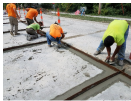
Partial-Depth Repairs
