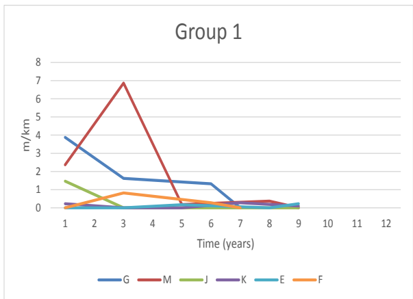
Figure A.11. High severity longitudinal cracking for Group 1
