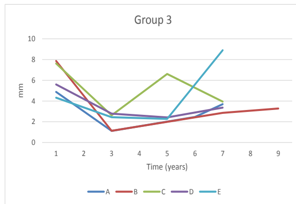
Figure B.2. Rutting on the right wheelpath for Groups 1, 2, and 3
