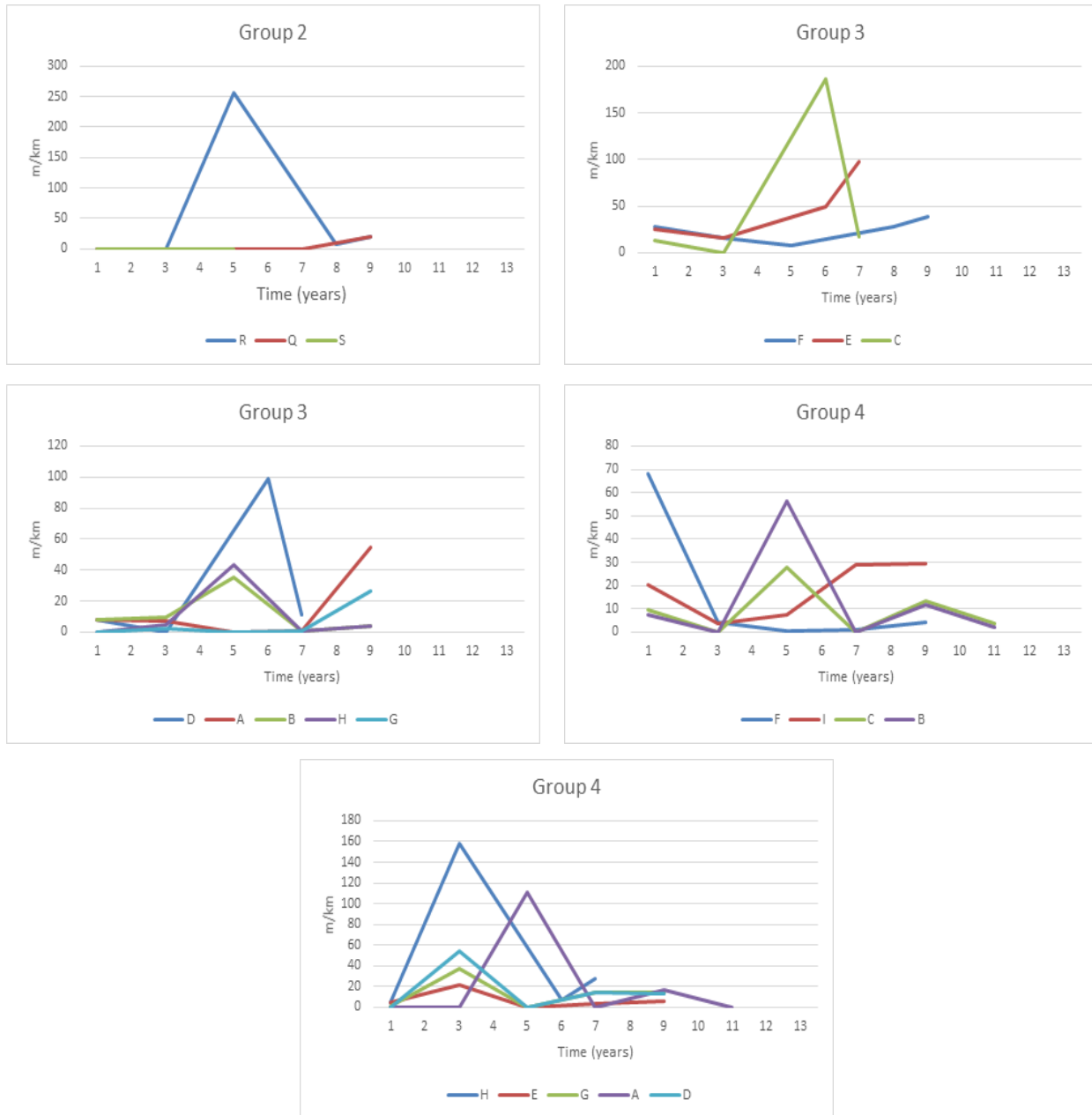
Figure 8. Moderate transverse cracking deterioration for Groups 2, 3, and 4
