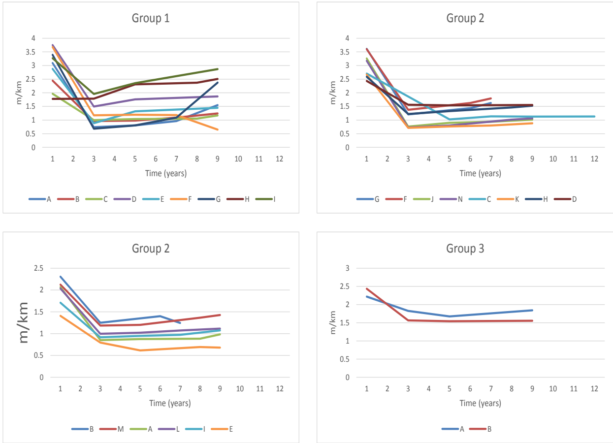
Figure A.16. IRI on the right wheelpath for Groups 1, 2, and 3
