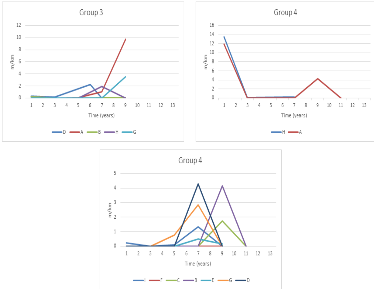
Figure 16. High longitudinal cracking deterioration for Groups 3 and 4
