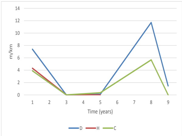
Figure C.13. High severity longitudinal cracking on wheelpath
