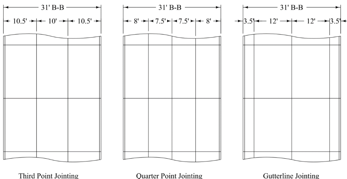
Figure 5G-2.05: 31 Foot B-B Pavements
