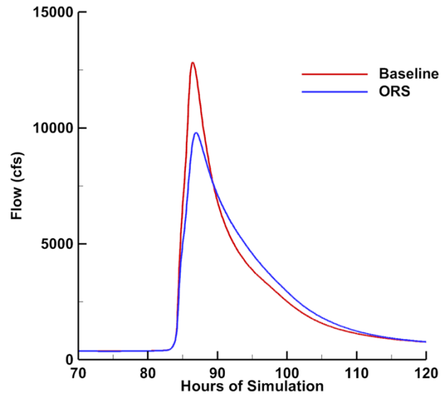
Figure 21. Peak flow comparison at an interior point in the Village of Van Horne – Prairie Creek watershed, showing modeled values (vertical axis) versus estimates from regionalization and regression equations (StreamStats) (left), and hydrographs at the watershed outlet depicting model predictions for the 50-year storm with ORS and without ORS (baseline) in place (right)
