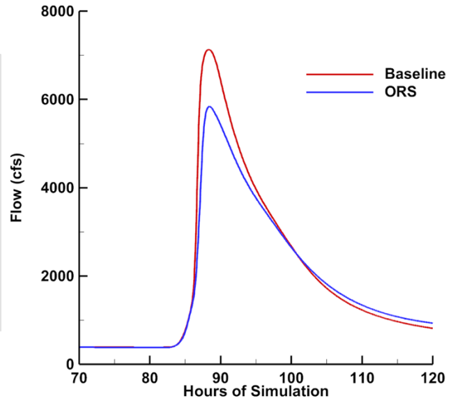
Figure 23. Peak flow comparison at the West Branch Mill Creek – Mill Creek watershed outlet, showing modeled values (vertical axis) versus estimates from regionalization and regression equations (StreamStats) (left), and hydrographs at the watershed outlet depicting model predictions for the 50-year storm with ORS and without ORS (baseline) in place (right)
