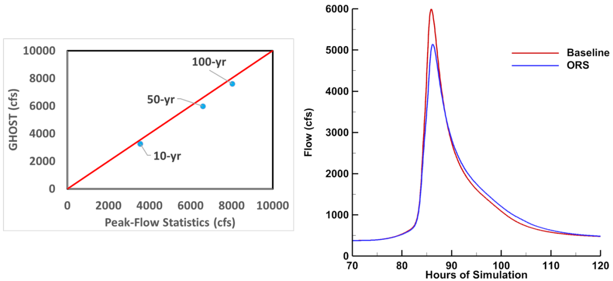
Figure 17. Peak flow comparison at the Bear Creek – Soap Creek watershed outlet, showing modeled values (vertical axis) versus estimates from regionalization and regression equations (StreamStats) (left), and hydrographs at the watershed outlet depicting model predictions for the 50-year storm with ORS and without ORS (baseline) in place (right)
