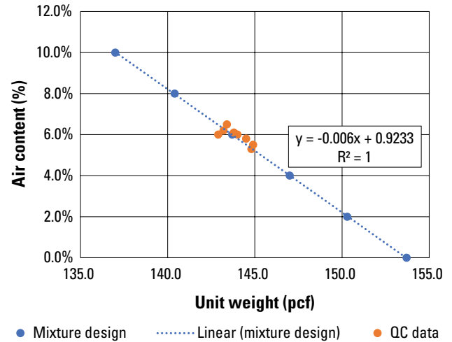
Figure 6.20. Relationship between design air content and design unit weight and between design values and measured values
