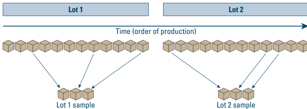
Figure 2.6. Random sampling
