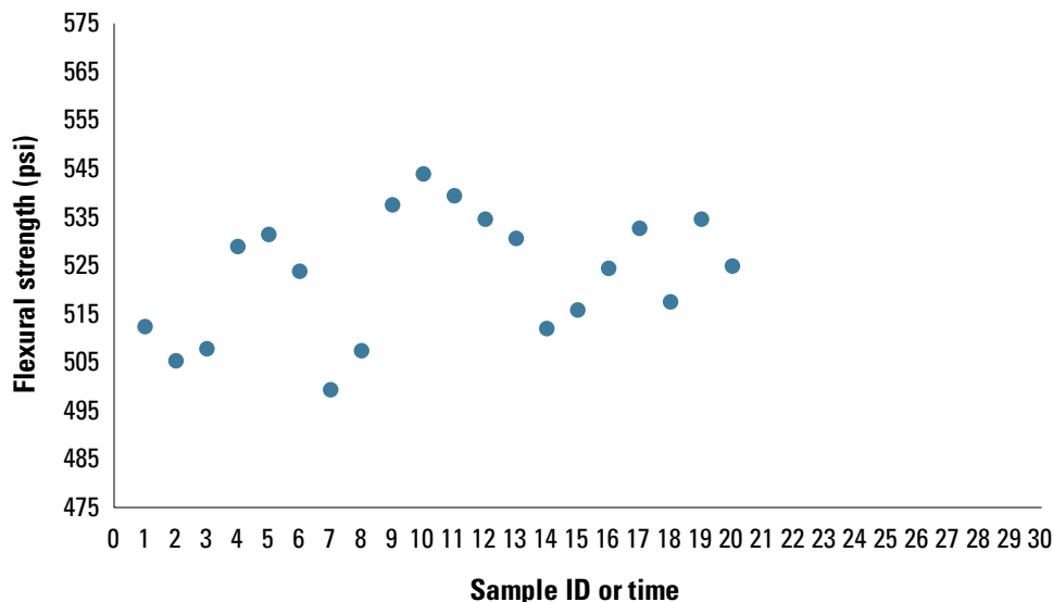
Figure 6.6. Run chart for the flexural strength of a concrete mixture
