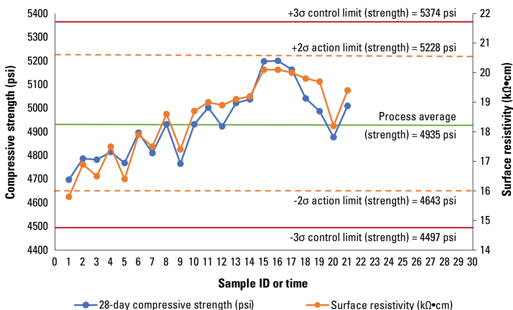
Figure 6.21. Control chart for compressive strength and surface resistivity
