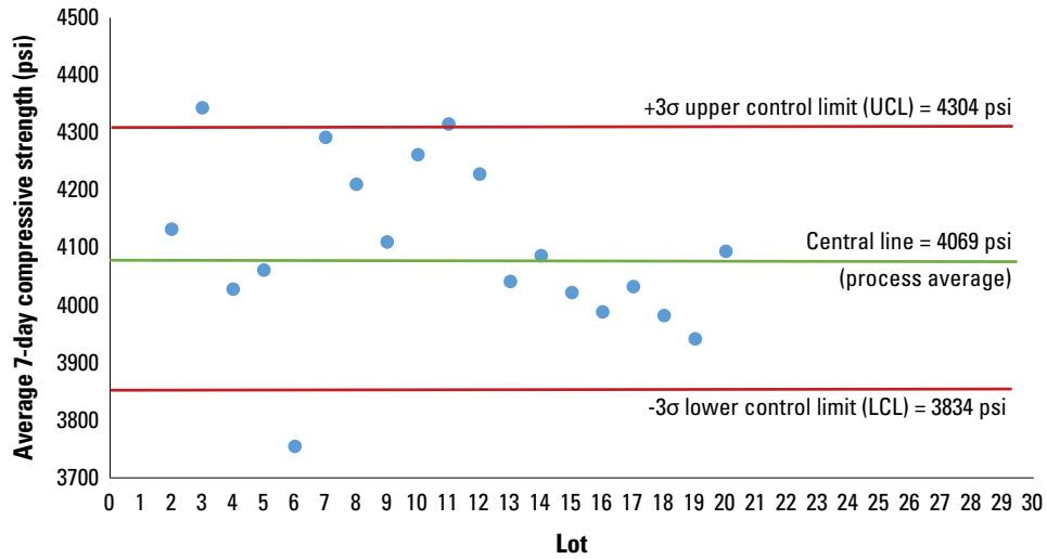
Figure E.3. \bar{X} chart with trial central line and control limits
