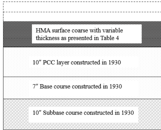
Figure 8. Structure of existing pavement
