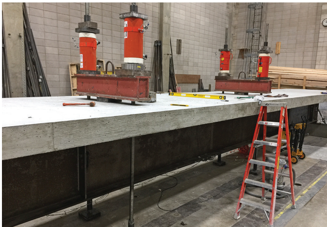
Loading setup for composite beam under 50% yield moment
