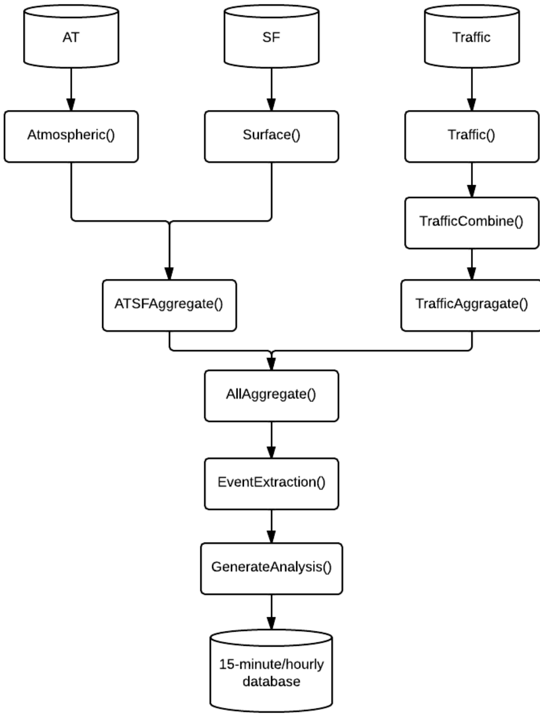
Figure 0.2 Data Processing Framework
