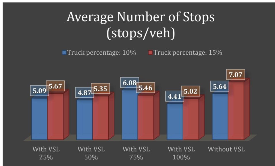
Figure 14. Average number of stops
