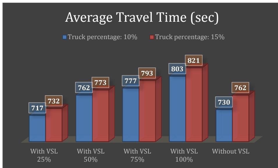
Figure 15. Average travel time
