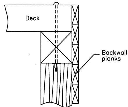
Thru-Bolt Abutment Connection Side view
