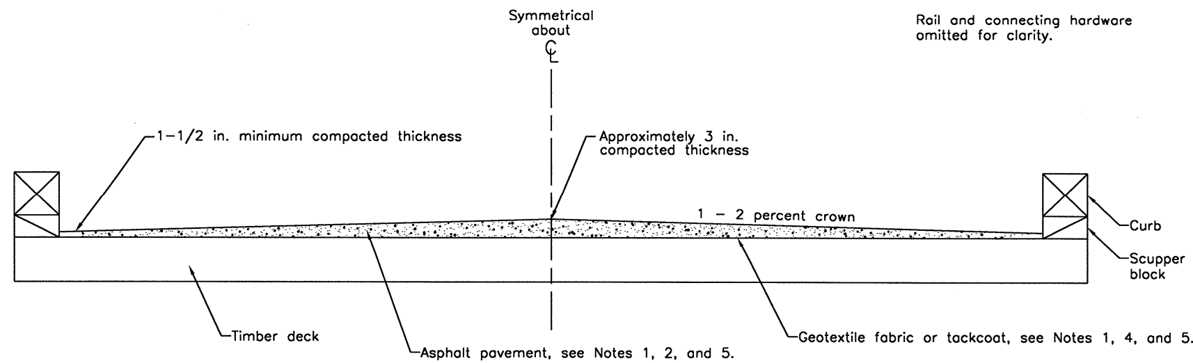
Cross-section view
