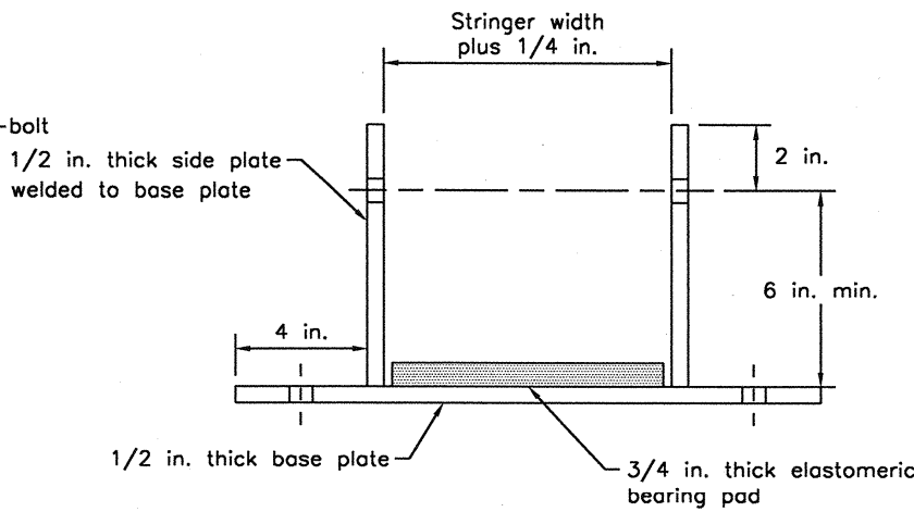
Steel Plate Bearing Shoe End view
