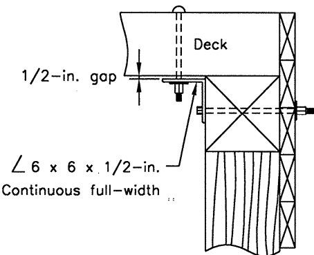
Steel Angle Abutment Connection Side view
