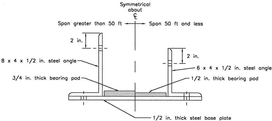
Steel Angle Bearing Shoe End view
