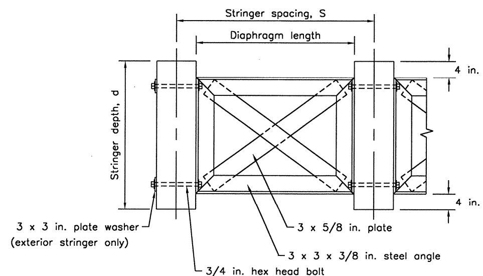
End view
