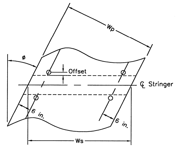
Attachment Spacing - End Panel Plan view
