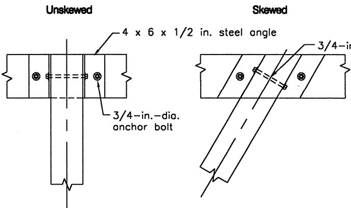
Bearing Clip Configuration Plan view
