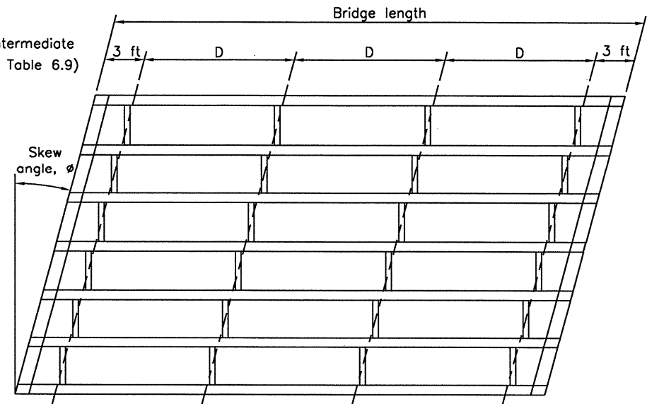
Skewed Bridges Plan view
