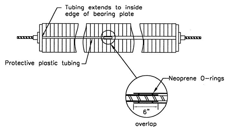
Protective PVC Tubing for Galvanized Bars Section view
