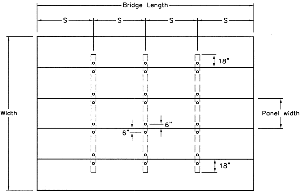
Transverse Stiffener Layout - Unskewed Crossings Plan View
