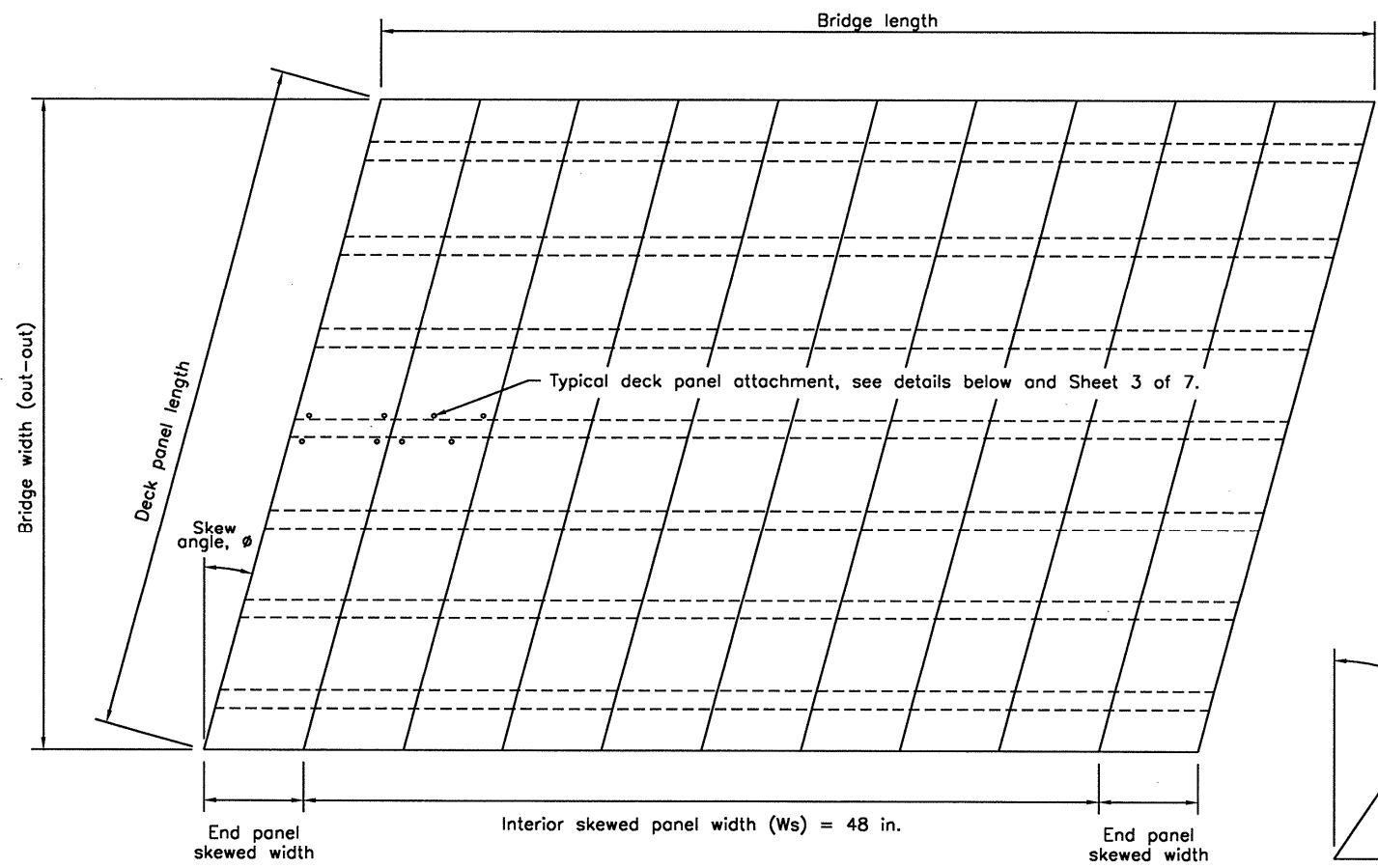
Plan View
