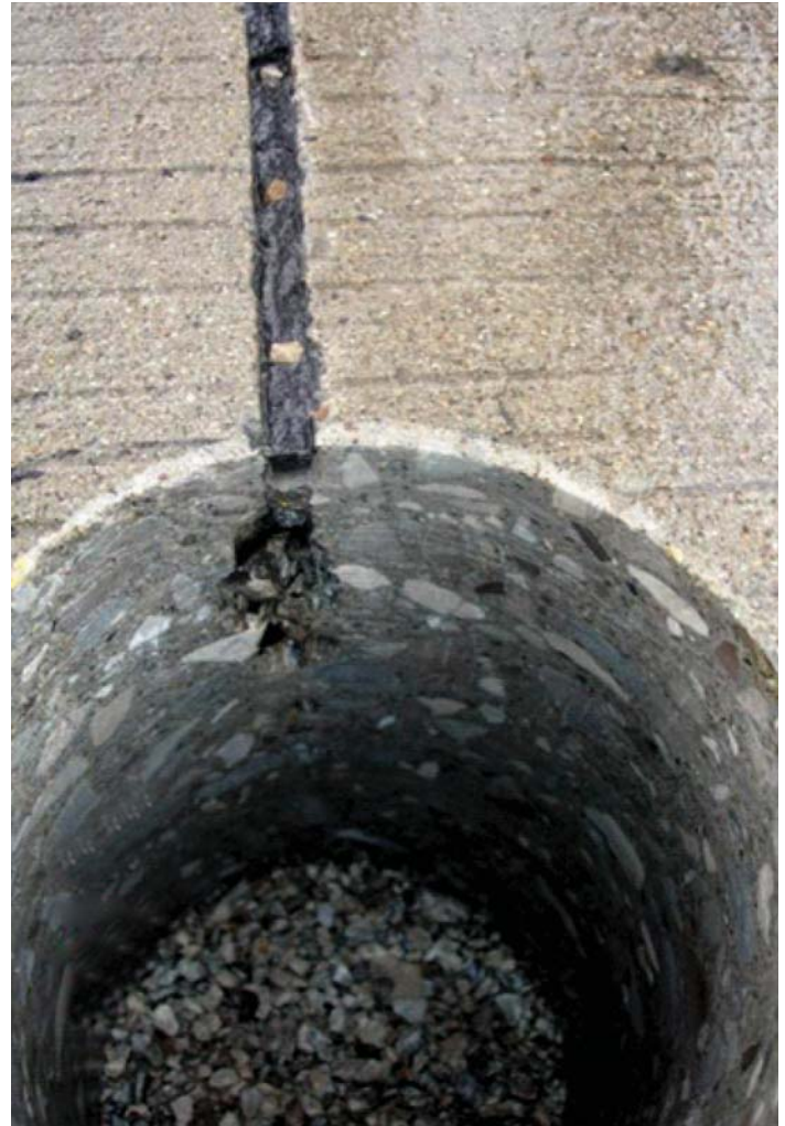
Figure 5. Example of damage occurring in a slab that has not cracked out
