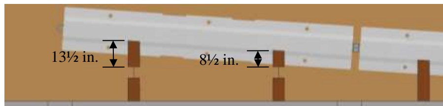
Figure 75. Blockouts Behind Posts Depths
