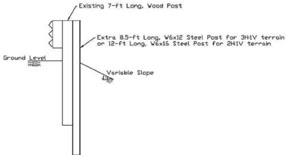
Figure 27. Driven-Post Design [30]
