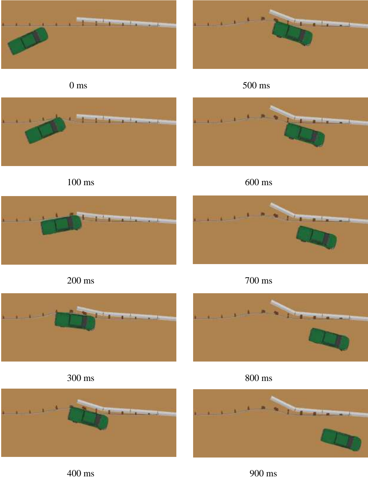
Figure 76. MGS with Blockouts Behind Posts Sequential, Impact Location No. 9
