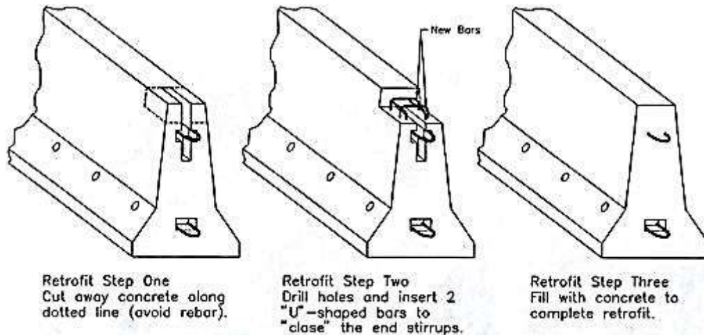
Figure 4. Retrofit to F-Shape PCB Sections [8]
