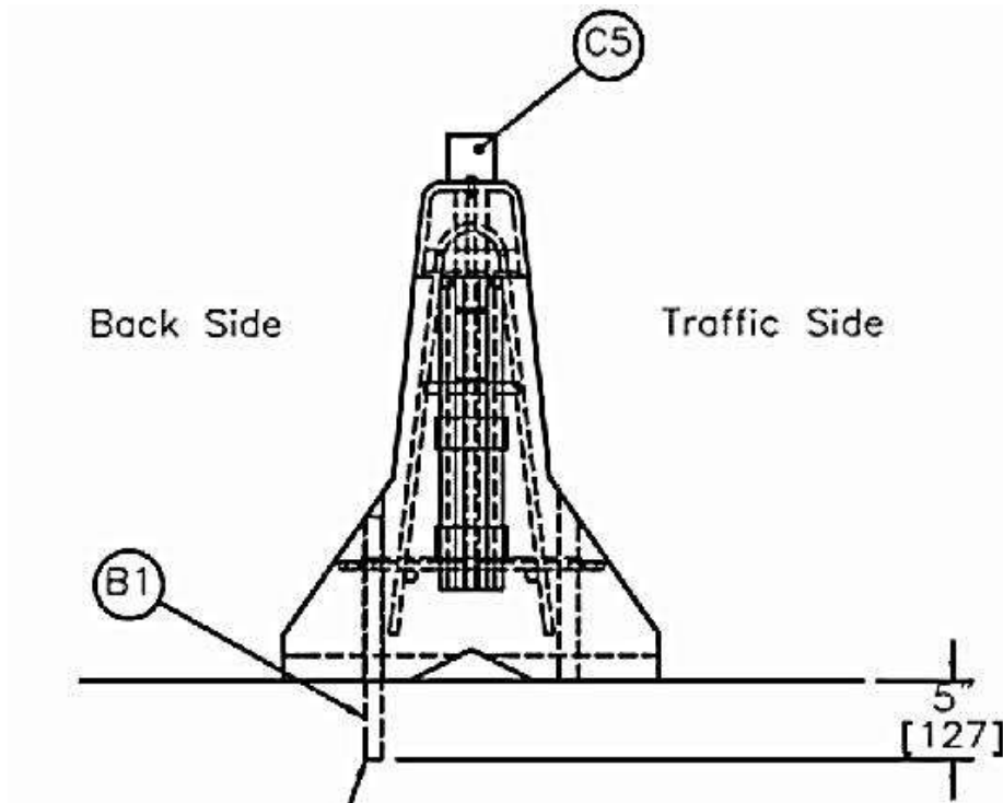
Figure 12. NYSDOT Pinned PCB Setup [15]
