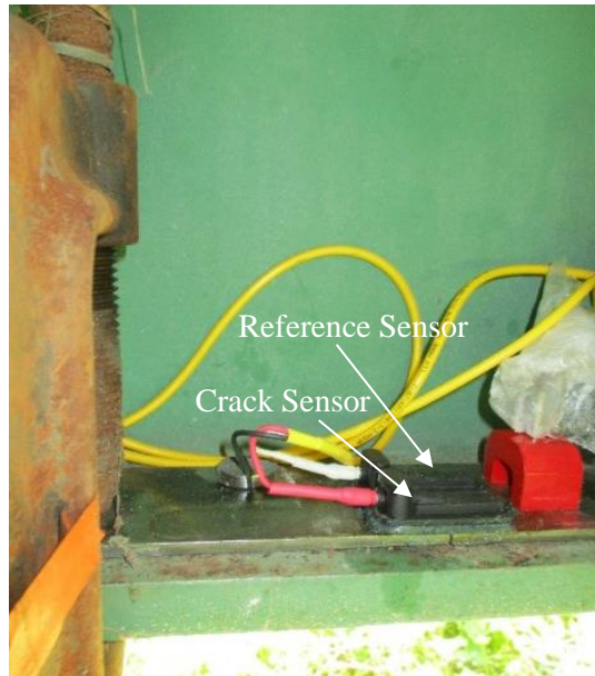
(b) Sensors on the sacrificial specimen
