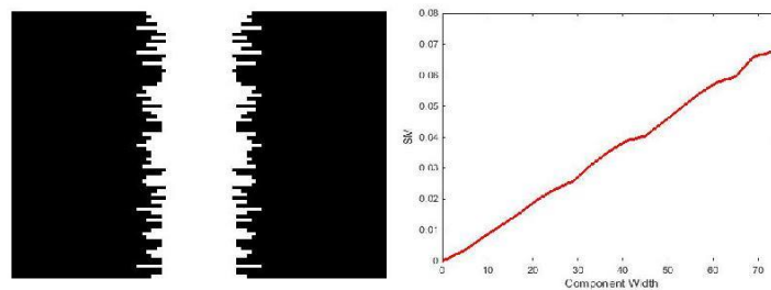
Figure 11. Relation between crack width and shape metric (SM): 25 pixel wide crack (left) and relation chart (right)
