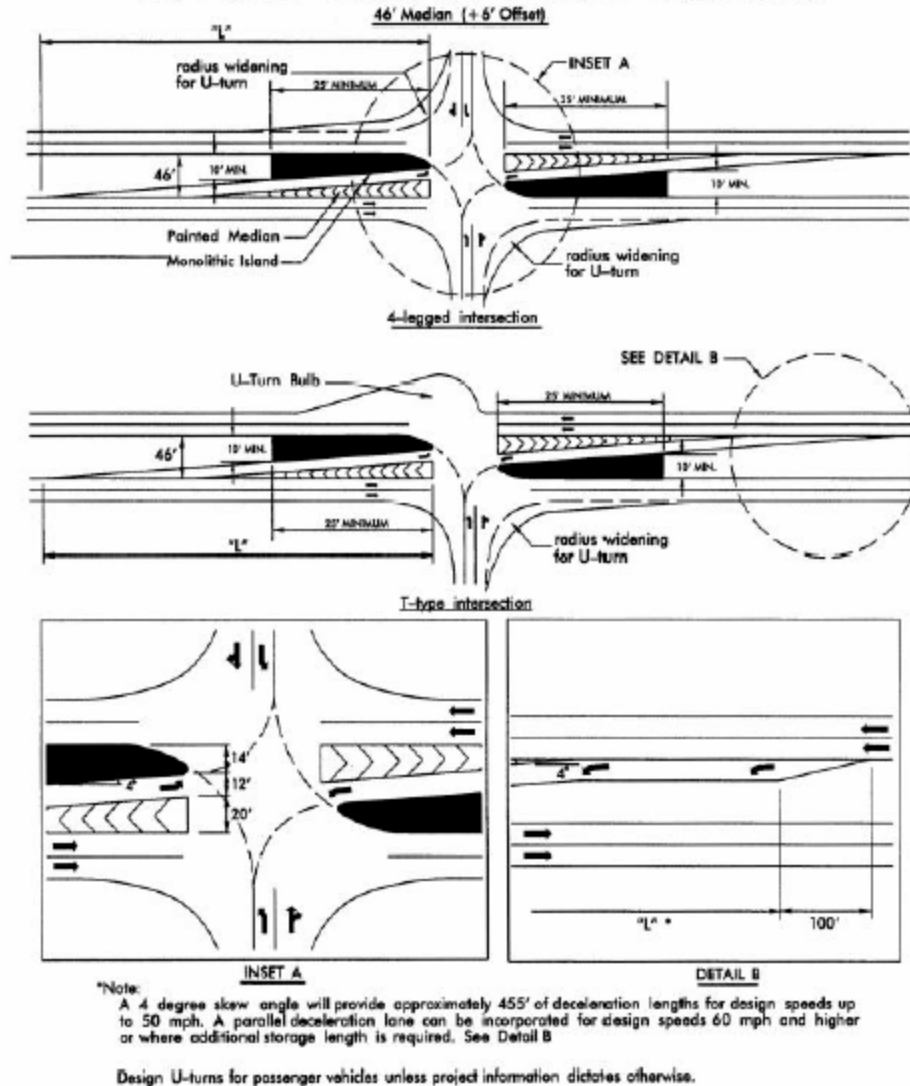
Figure 3.14. Offset left-turn design
