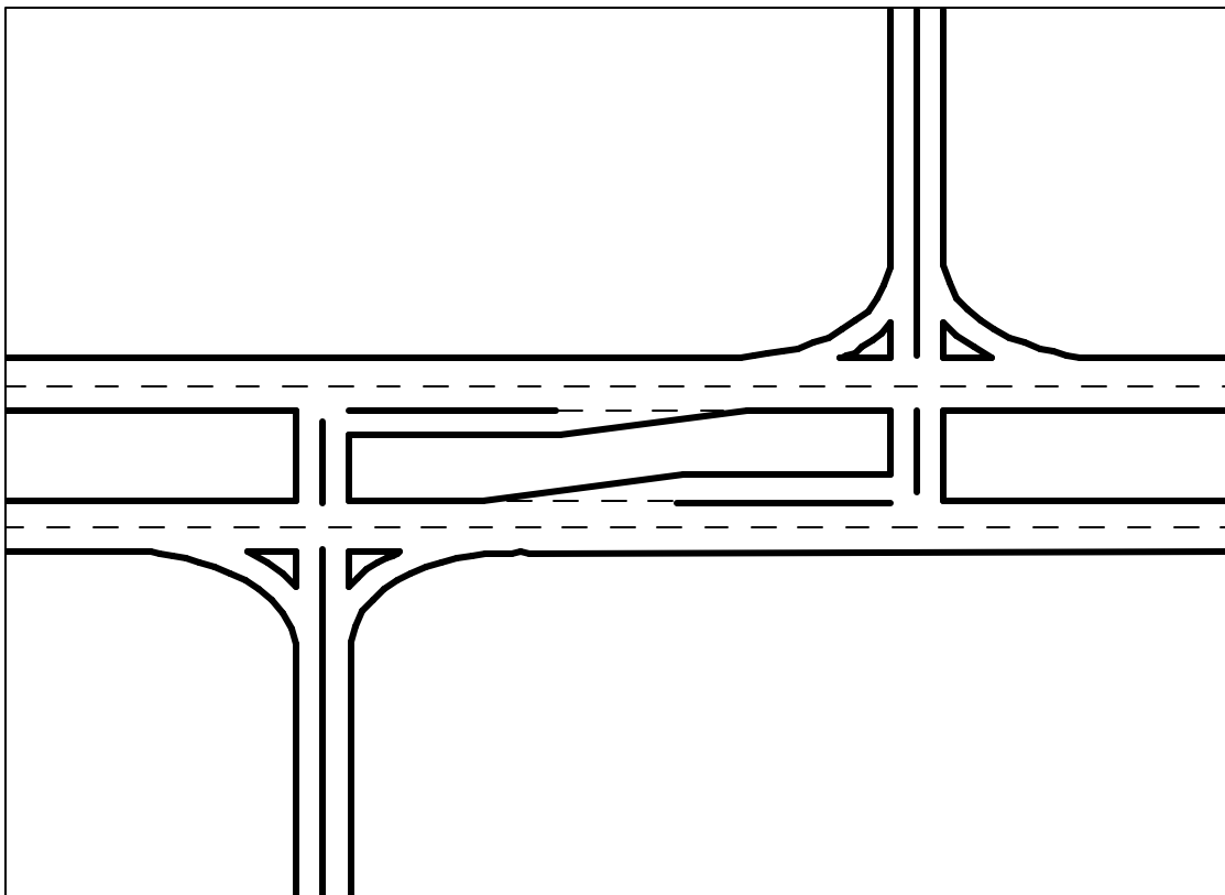
Figure 2.9. Offset T-intersection
