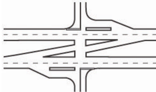
Figure 2.4. Intersection with offset right and offset left-turn lanes
