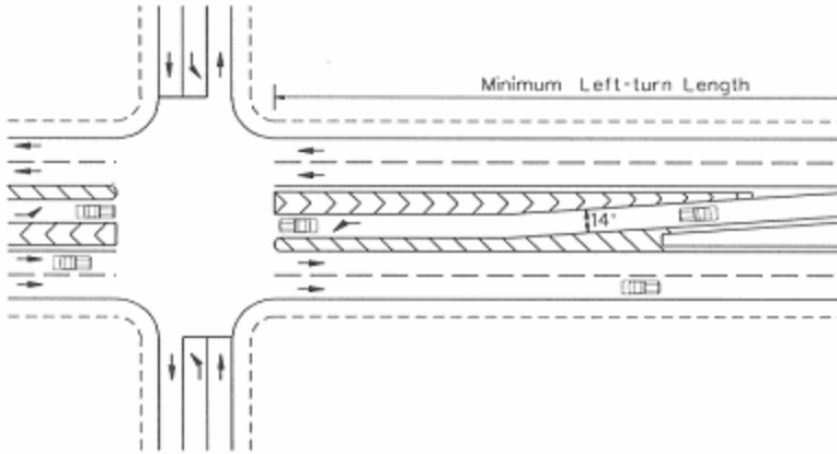
(b) PARALLEL-OFFSET TURN LANE
