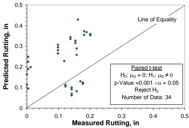
Figure 27. Verification testing results for rutting and IRI - HMA over HMA pavements in Iowa
