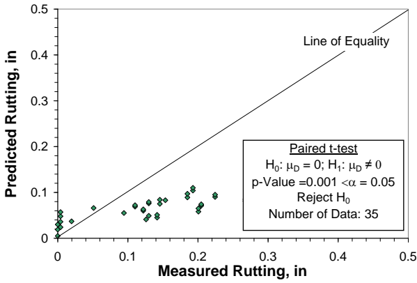
Figure 26. Verification testing results for rutting and IRI - HMA over JPCPs in Iowa
