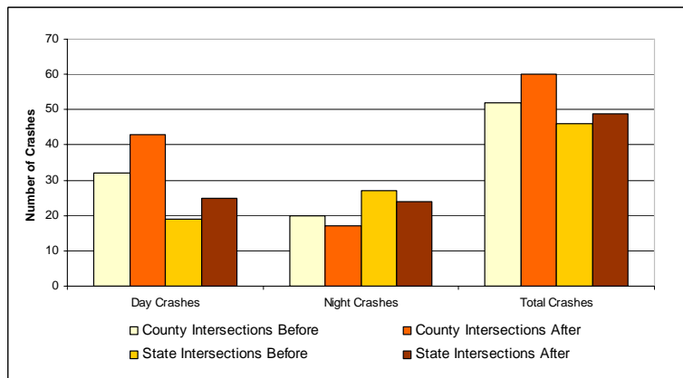
Figure 5.2. Crash frequency
