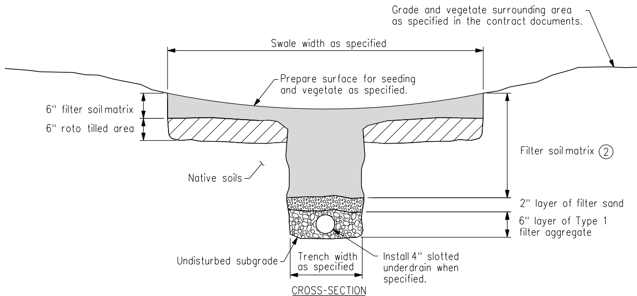
CROSS-SECTION
