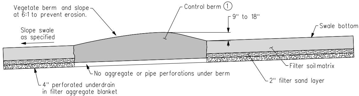
SWALE PROFILE
