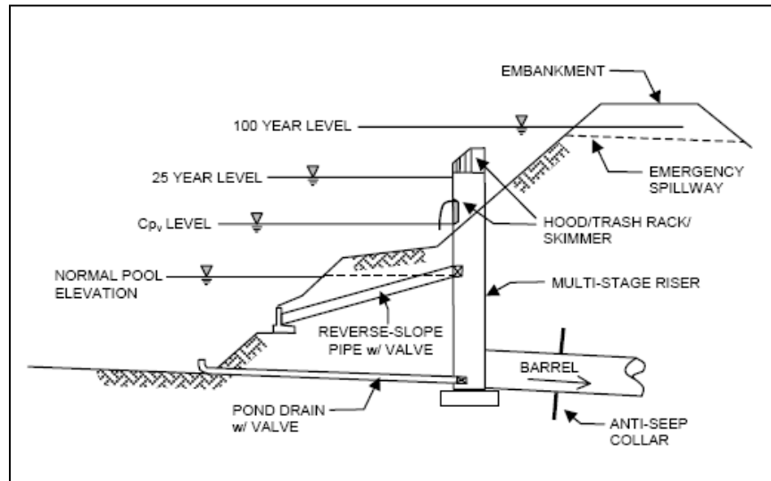
Figure 4: Typical multiple outlet structure for wet detention basin
