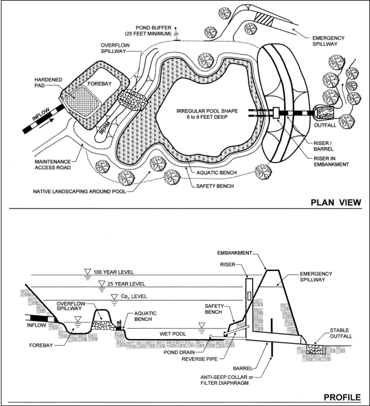
Figure 5: Example schematic of wet detention basin (wet pond)
