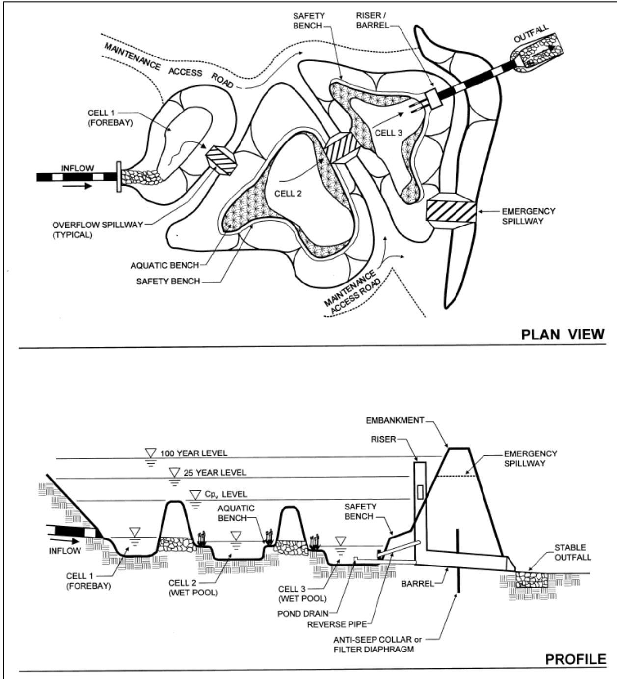
Figure 8: Example schematic of multiple pond system
