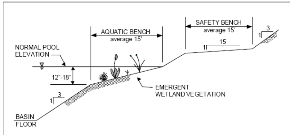
Figure 3: Typical stormwater pond geometry criteria
