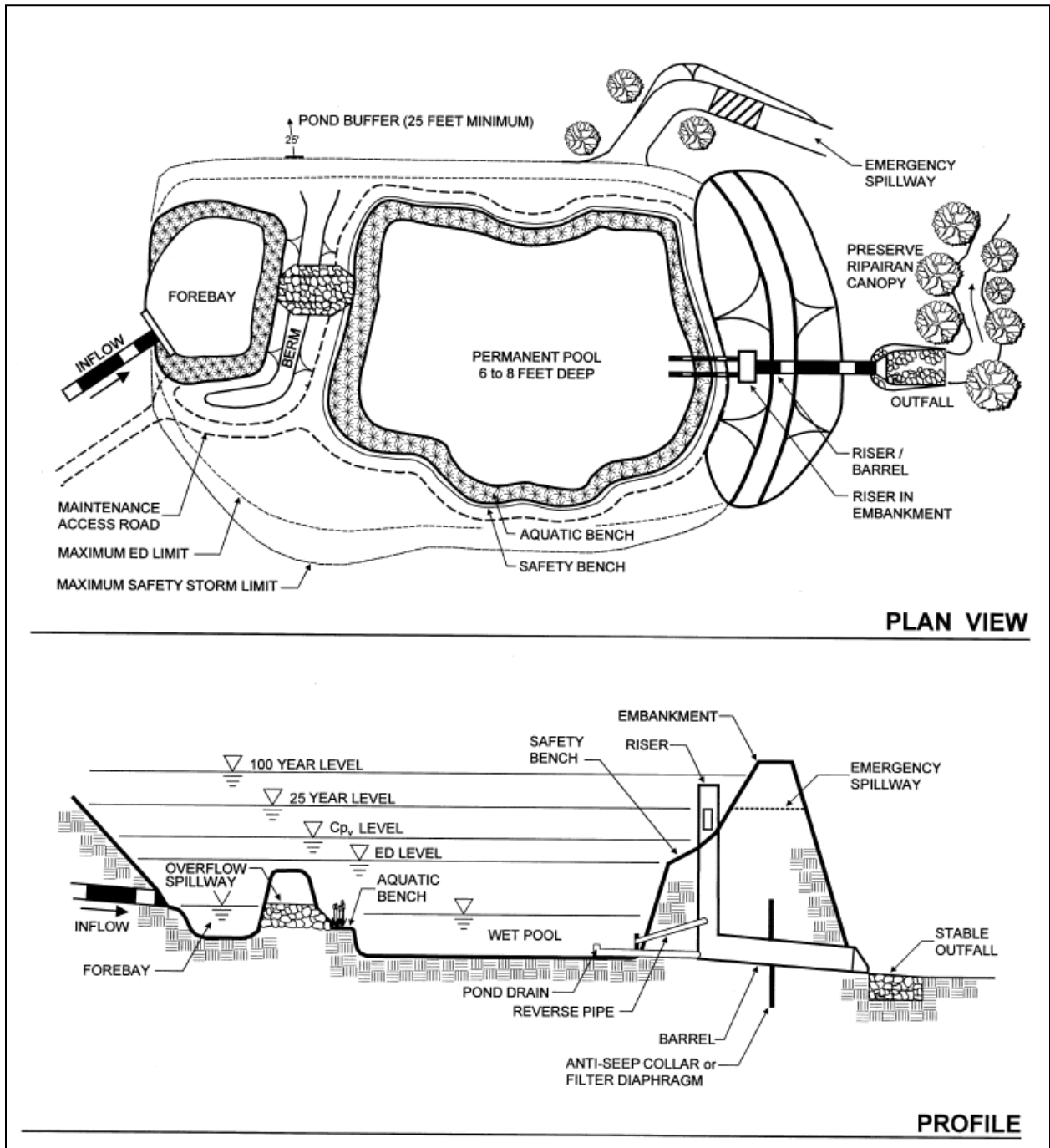
Figure 6: Example schematic of wet extended detention basin (ED wet pond)
