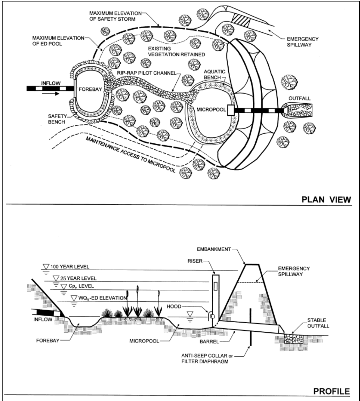
Figure 7: Example schematic of micro-pool extended detention pond
