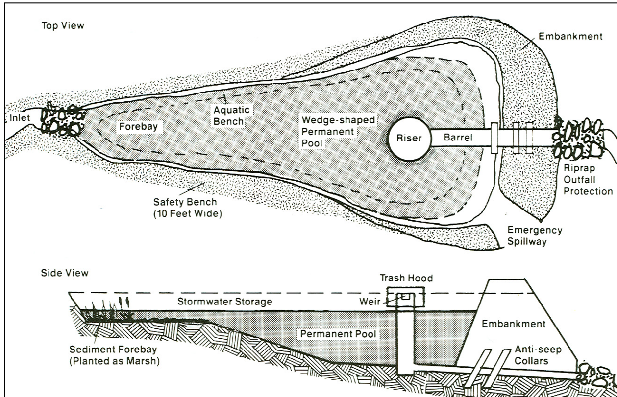
Figure 1: Schematic of wet detention basin (wet pond)
