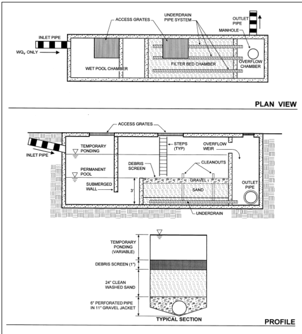
Figure 2: Underground sand filter
