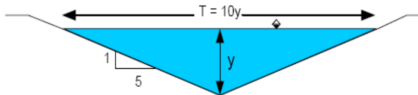
Figure 2: Schematic for Muskingum-Cunge routing example
